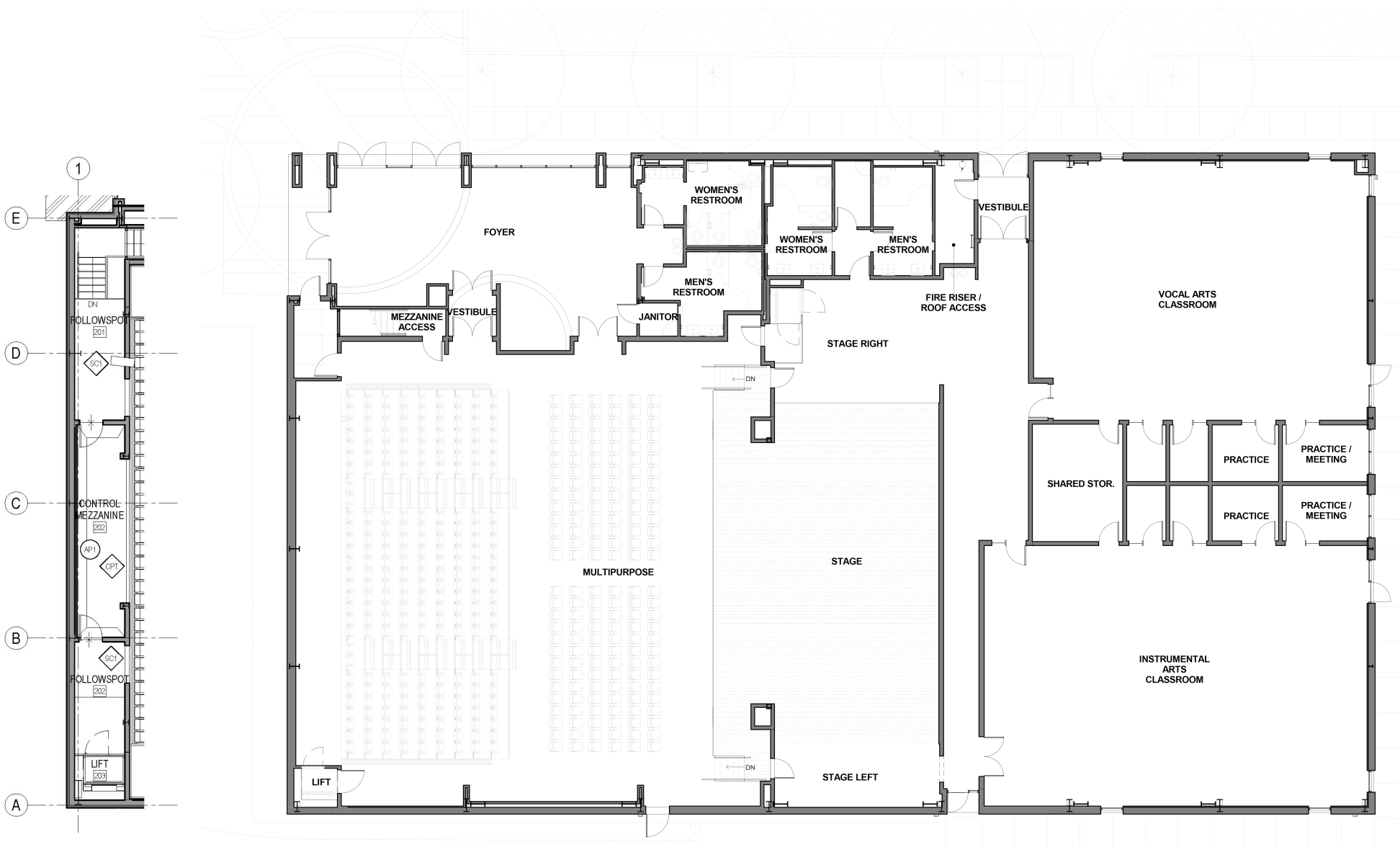
② MEZZANINE FLOOR PLAN - FINISH 1/8" = 1'-0"
